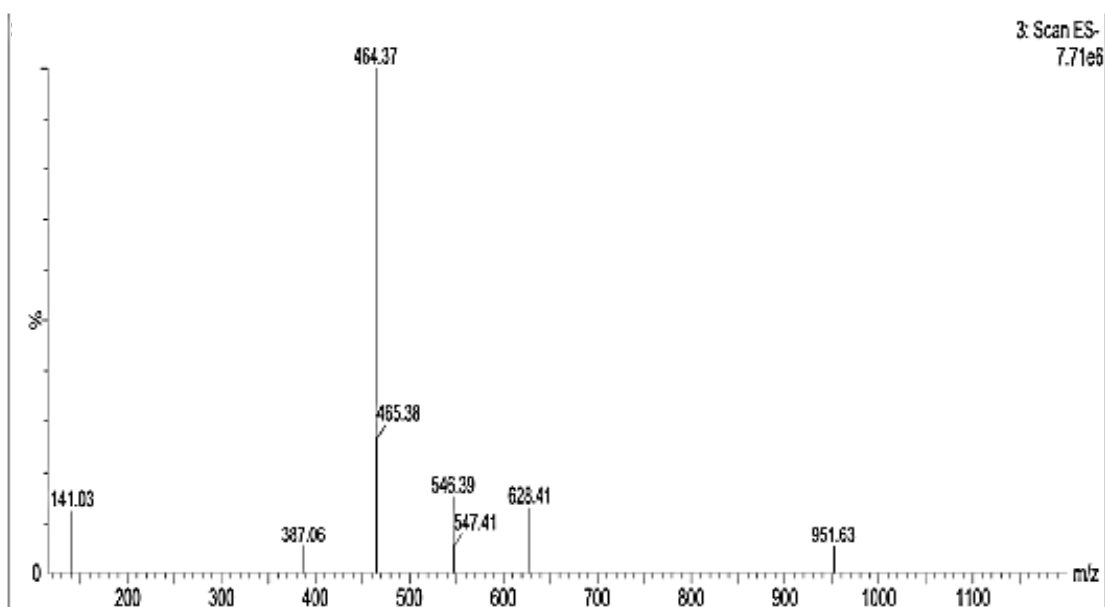
Mass by LCMS (ESI negative ion mode)
