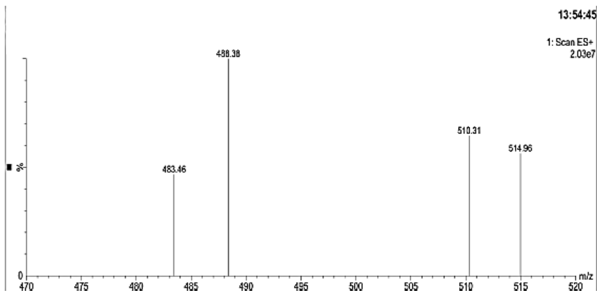
Mass by LCMS (ESI positive ion mode)
